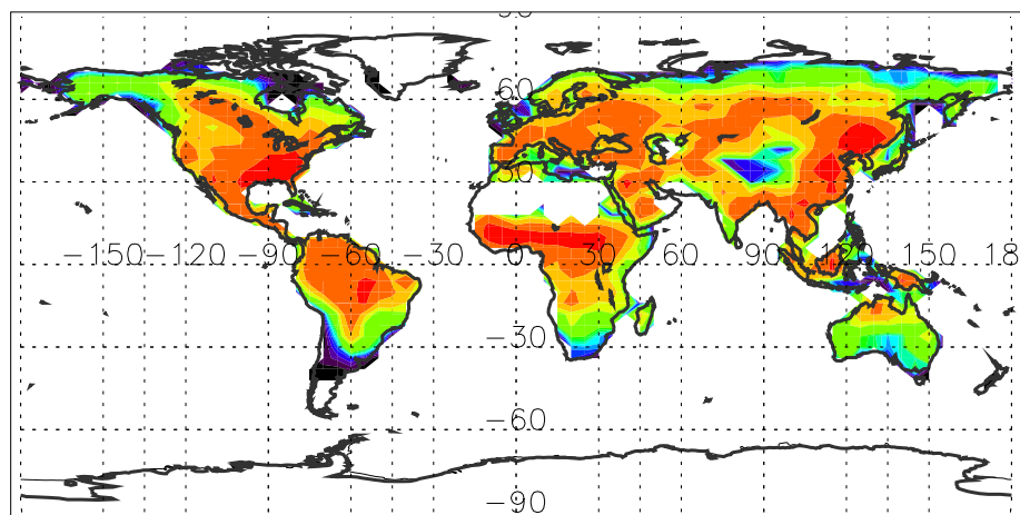
Isoprene emission (mgC/m 2 month)07
