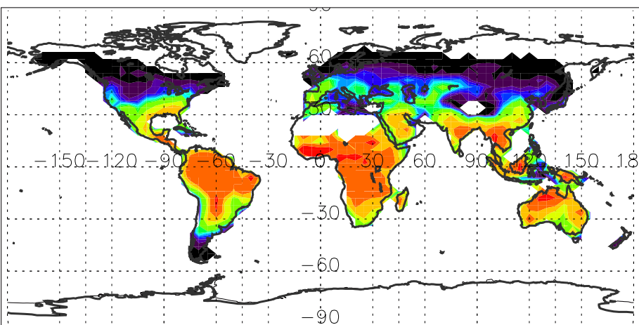
Isoprene emission (mgC/m 2 month)04
