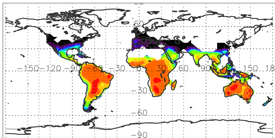
Isoprene emission (mgC/m 2 month)03
