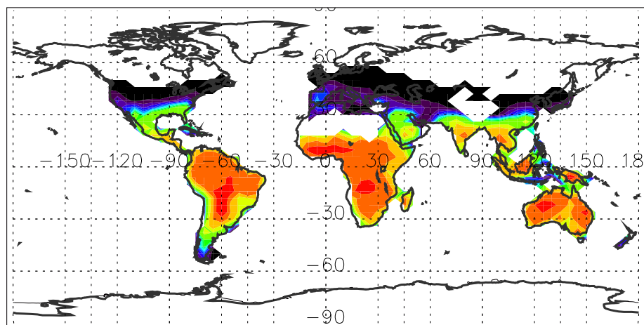
Isoprene emission (mgC/m 2 month)11
