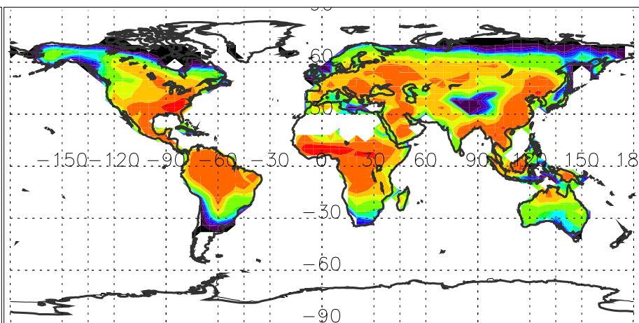
Isoprene emission (mgC/m 2 month)08
