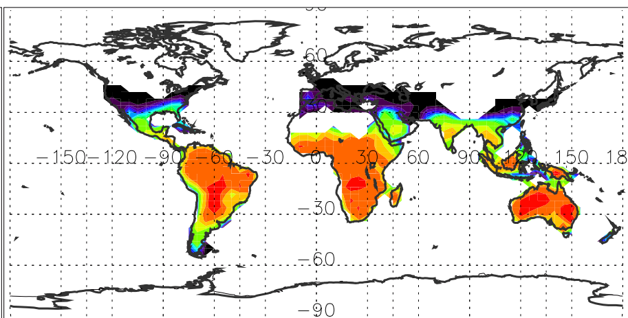
Isoprene emission (mgC/m 2 month)12
