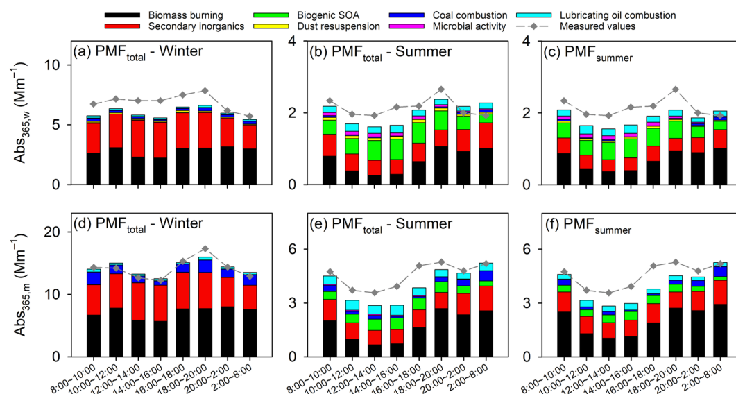
Figure 5. Diurnal distributions of factor contributions to (a–c) Abs_{365,w} and (d–f) Abs_{365,m} in winter and summer, derived from PMF_{total} and PMF_{summer} solutions.
