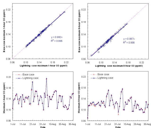
Fig. 5. Temporal evolution of domain-wide daily maximum 1-h (left panel) and 8-h (right panel) \text{O}_3 values with versus without lightning for July–August 2004 (One grid with the maximum 1-h and 8-h \text{O}_3 is selected throughout the whole domain for each day).
