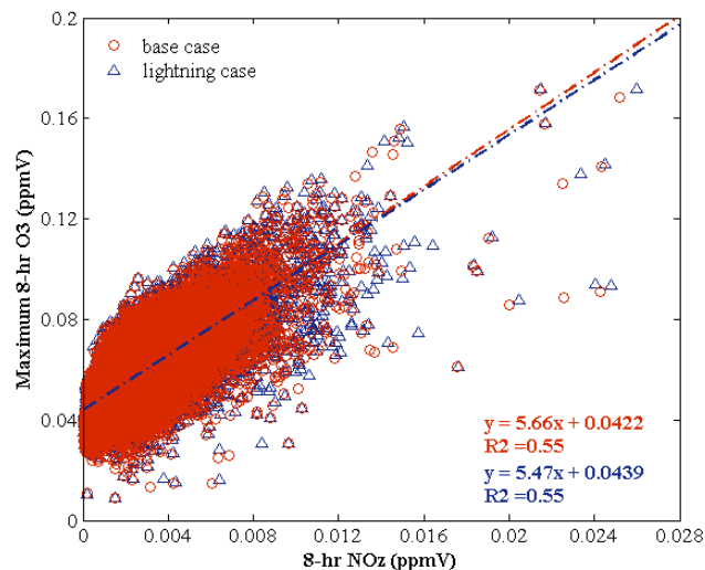
Fig. 11. Daily 8-h maximum O 3 versus corresponding daily 8-h NO z (NO y –NO x ) for grids with AIRS Ozone monitoring stations for July–August 2004. Shown are results for the base case (no lightning emissions) and lightning case.
