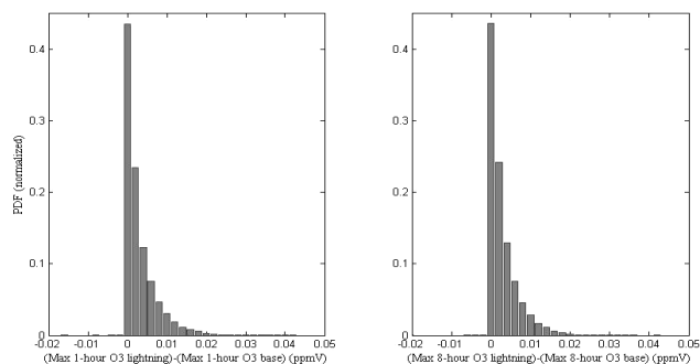
Fig. 6. Distribution of the difference (Lightning case – Base case) in daily 1-h and 8-h maximum O 3 values for grids with AIRS ozone monitoring stations for July–August 2004.
