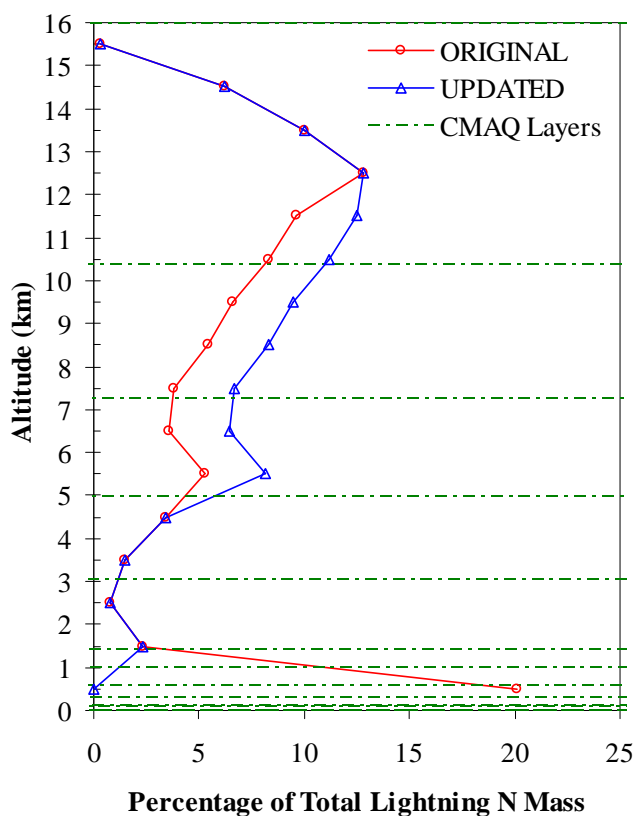
Fig. 2. Original and updated vertical profiles used for allocating lightning NO x emissions into model layers.
