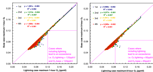
Fig. 8. The 1st, 2nd, 3rd and 4th highest 1-h (left panel) and 8-h (right panel) maximum O 3 values for model grids with AIRS ozone monitoring stations for July–August 2004. (2768 (692×4) points).
