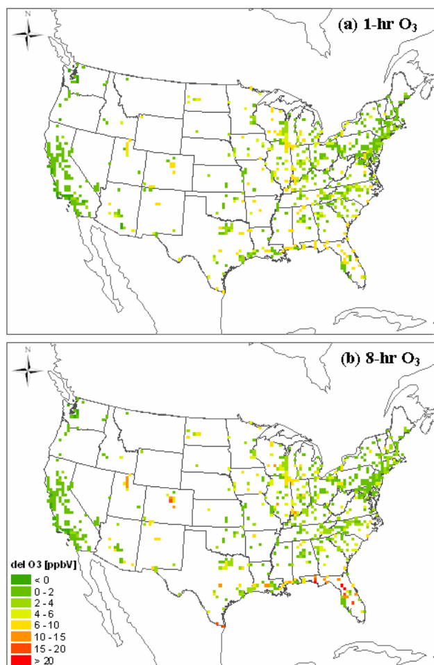
Fig. 10. Differences in (a) 1-h and (b) 8-h maximum O 3 values for model grids with AIRS Ozone monitoring stations for July–August 2004 (Difference in maximum daily first highest values are selected for each grid).
