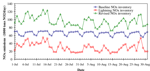
Fig. 3. Domain-wide baseline, lightning, and revised NO x emissions (as tons NO 2 /day) for July–August 2004.
