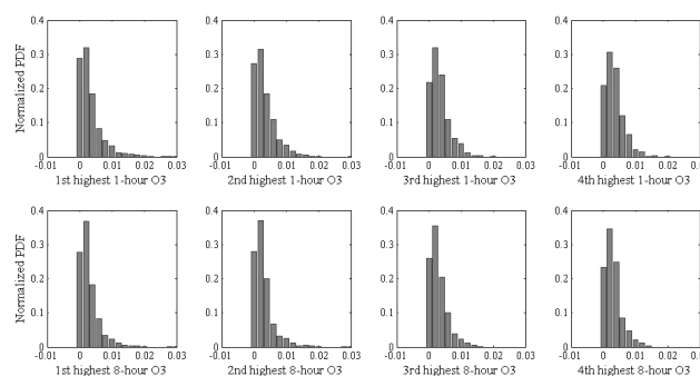
Fig. 9. Distribution of the difference (Lightning case – Base case) in the 1st, 2nd, 3rd and 4th highest 1-h (top) and 8-h (bottom) maximum O 3 values for grids with AIRS Ozone monitoring stations (PDF's are normalized and differences in units of ppmv).
