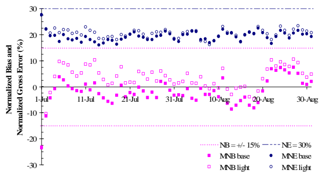
Fig. 1. Domain-wide daily normalized bias and error for 8-h O 3 in CMAQ when compared with AIRS, CASTNET and SEARCH O 3 measurements (for all pairs of O 3 >40 ppbv).
