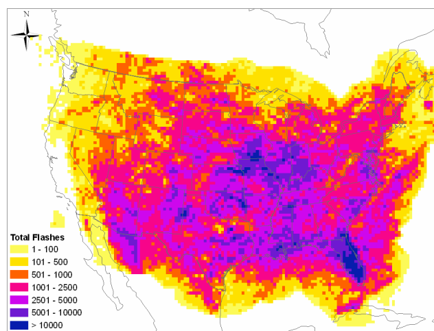
Fig. 4. Domain-wide lightning intensity map for July–August 2004.
