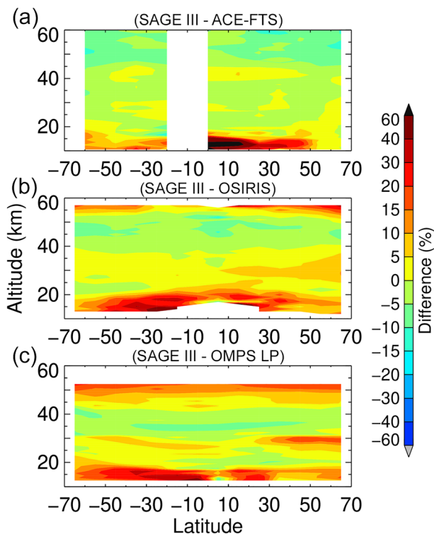
Figure 10. Mean differences between SAGE III/ISS AO3 ozone and correlative (a) ACE-FTS, (b) OSIRIS, and (c) OMPS LP (bottom panel) measurements. Differences are represented as (\text{SAGE}-\text{other})/\text{other} * 100\% .
