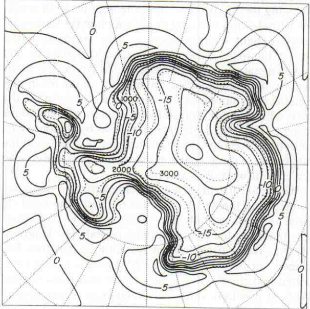
FIG. 14. As in Fig. 9 except for 10 days of model integration.
