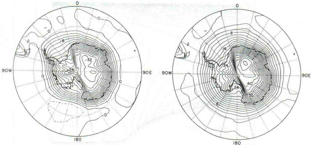
FIG. 5. Mean monthly surface temperature differences. April minus January 1987 (left) and December minus September 1990 (right) based on ECMWF analyses.
