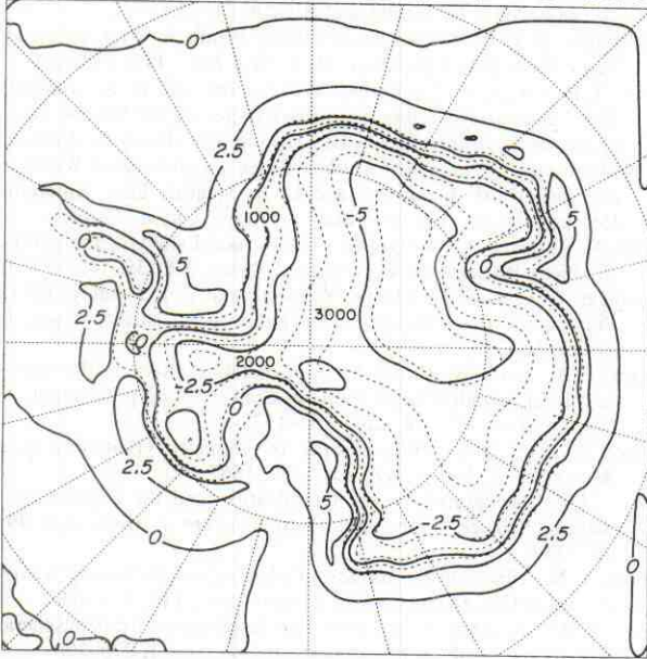
FIG. 13. Surface pressure changes (hPa) from start of three-dimensional model experiment after 2 days of model integration.
