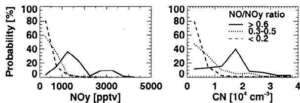
Figure 4. Percentage probability distributions for CN (binned per 5000 \text{cm}^{-3} ) and \text{NO}_y (binned per 500 pptv) in the upper troposphere for data with \text{NO}/\text{NO}_y ratios of <0.2 , 0.3\text{--}0.5 , and >0.6 mol/mol. Aircraft plumes are filtered out.
